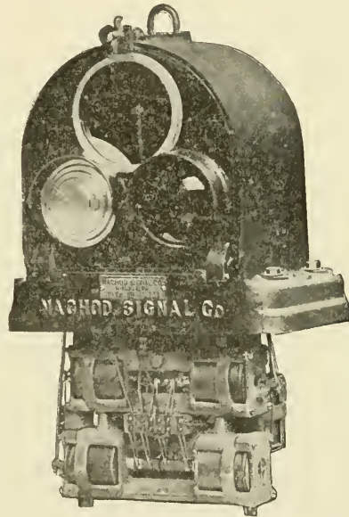
Fig. 217. Box Showing Operating Mechanism
